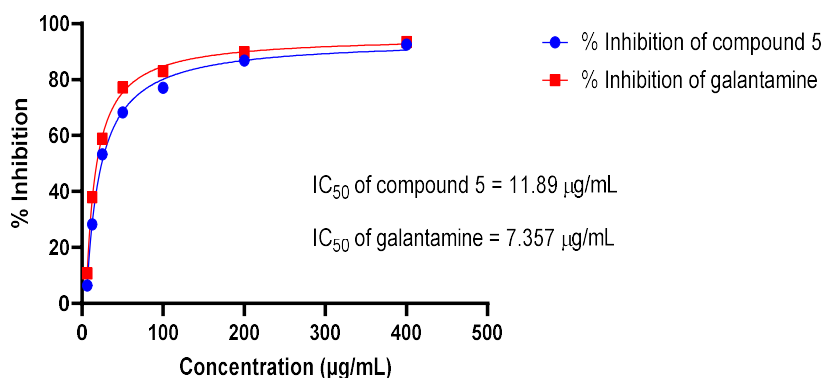
Figure 2: The IC_{50} value of galantamine versus compound 5 against AChE
